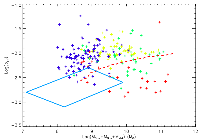
Figure 17. Total baryonic mass against the effective yield ( p_{\text{eff}} ). Red is for galaxies with type earlier than Sa, green for type Sa/Sb, yellow for type Sc and blue for galaxies later than Sc and dwarfs. The red dashed line shows the median relation for \sim 53 000 SDSS galaxies taken from Tremonti et al. (2004). The blue box represents the area occupied by the Virgo cluster dwarf irregular galaxies studied by Lee et al. (2003).
