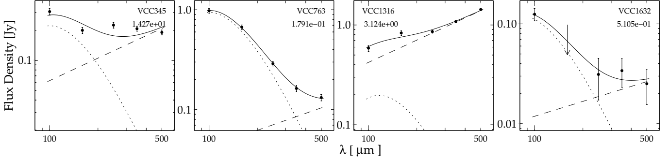
Fig. 5. Modified black-body fits to the HeViCS fluxes for the detected ETG with synchrotron emission. The synchrotron component is shown as a dashed line, the dust one as a dotted line. The reduced \chi^2 of each fit is listed under the object name. Upper limits to the fluxes are shown by downward arrows.
