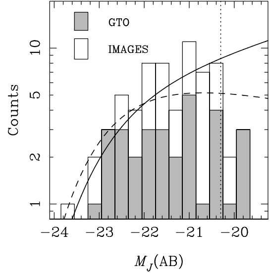
Fig. 1. Number counts (in logarithmic scale) of selected galaxies versus AB absolute magnitude in J -band. The GTO sample refers to Flores et al. (2006); the IMAGES sample refers to this paper. The vertical dotted line indicates the limit of the IMAGES program. Two luminosity functions derived from Pozzetti et al. (2003) are shown (full line: z = 0.5 ; dashed line: z = 1 ). The galaxies of our sample have redshifts ranging from z = 0.4 to z = 0.75 . This implies that the combined sample of 63 galaxies with M_J(\text{AB}) \leq -20.3 is representative of galaxies with stellar masses larger than 1.5 \times 10^{10} M_{\odot} at z \sim 0.6 .
